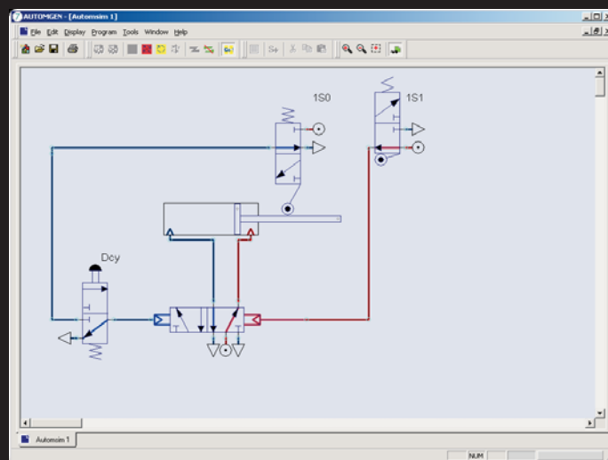
Pneumatic simulation
